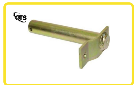
ITEM NAME LINKAGE PIN / BUCKET PIN MATERIAL EN - 19 SIZE 35 X 195 WITH BEND PROFILE PLATE WELDED TREATMENT & FINISH INDUCTION HARDENED & GROUND
