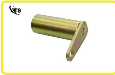
ITEM NAME LINKAGE PIN / BUCKET PIN MATERIAL EN - 19 SIZE 60 X 155 WITH PROFILE PLATE WELDED TREATMENT & FINISH HARDENED TEMPERED & GROUND
