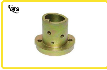
ITEM NAME CAM HAUSING MATERIAL EN - 19 SIZE TREATMENT & FINISH CASE CARBORISED, HARDENED & TEMPERED-58-60 HRC
