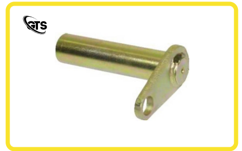
ITEM NAME LINKAGE PIN / BUCKET PIN MATERIAL EN - 8 SIZE 35 X 145 WITH ELLIPTICAL PROFILE PLATE WELDED TREATMENT & FINISH INDUCTION HARDENED & GOLDEN PLATED
