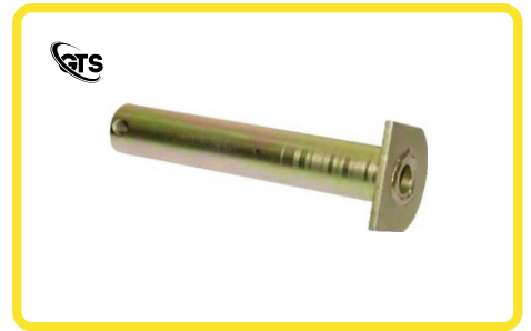
ITEM NAME LINKAGE PIN / BUCKET PIN MATERIAL EN - 8 SIZE 38 X 228 WITH PROFILE PLATE WELDED TREATMENT & FINISH INDUCTION HARDENED & GOLDEN PLATED
