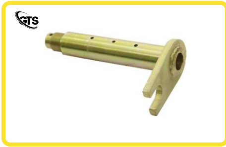
ITEM NAME LINKAGE PIN / BUCKET PIN MATERIAL EN8 - D SIZE 30 X 170 WITH FORK PROFILE PLATE WELDED TREATMENT & FINISH INDUCTION HARDENED & GOLDEN PLATED
