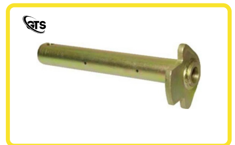
ITEM NAME LINKAGE PIN / BUCKET PIN MATERIAL EN - 8 SIZE 35 X 250 WITH ELLIPTICAL PROFILE PLATE WELDED TREATMENT & FINISH INDUCTION HARDENED & GOLDEN PLATED
