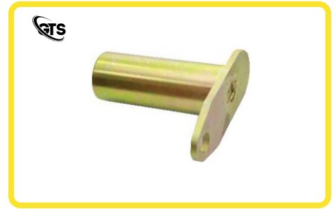
ITEM NAME LINKAGE PIN / BUCKET PIN MATERIAL EN - 19 SIZE 60 X 155 WITH FORK PROFILE PLATE WELDED TREATMENT & FINISH INDUCTION HARDENED & GOLDEN PLATED
