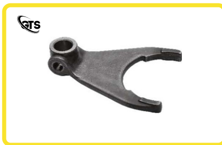
ITEM NAME FORK MATERIAL EN - 8D INVESTMENT CASTING SIZE BORE 15.80 X 90 TREATMENT & FINISH PADS INDUCTION HARDENED
